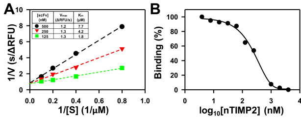
Figure 5. Inhibition mechanism of 9C1. (A) Lineweaver–Burke plots of cdMMP-9 in the presence of 125-, 250- and 500-nM scFv were developed. (B) Competitive ELISA with nTIMP-2.
